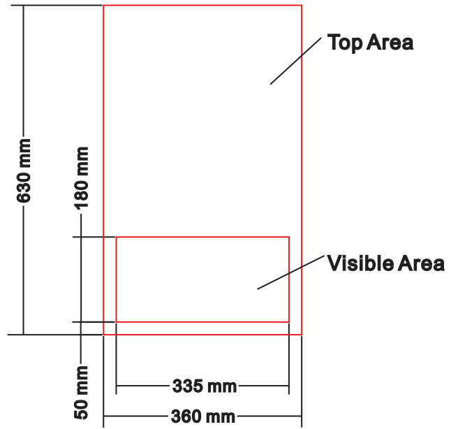
Top Front Panel
